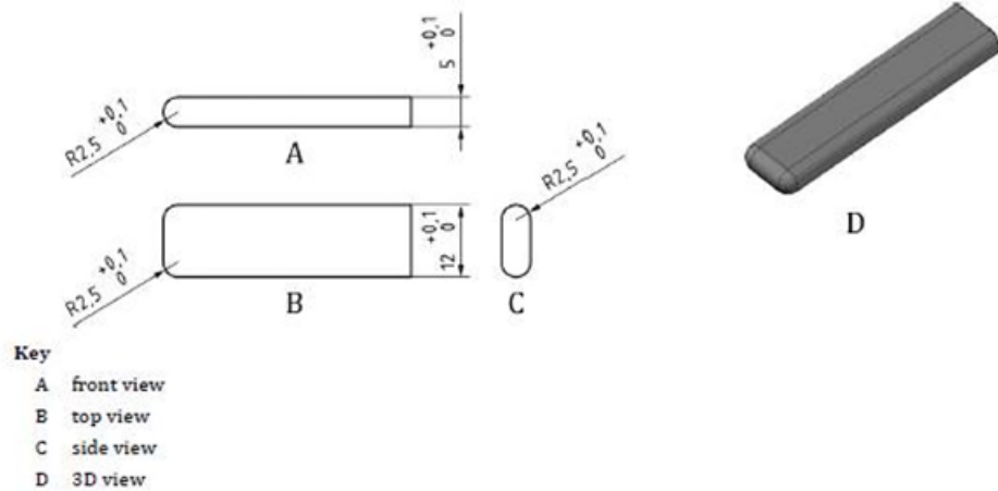
Figure 3 — Shape assessment probe
